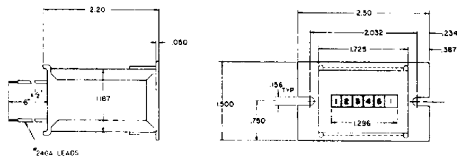
T12D62B07 Flange Mount
