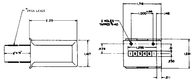
T12D62B02 Back of Panel Mount Without Legs
