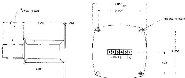
T12B62B NEMA Bezel Panel Mount
