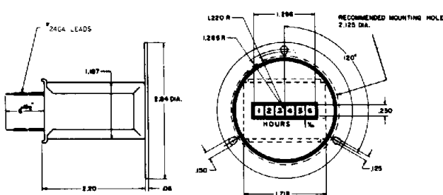
T12C62B Base Mount
