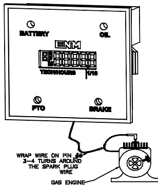
TACH/HOUR METER CONNECTION
